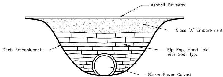
TYPICAL STORM CULVERT RIP RAP DETAIL
