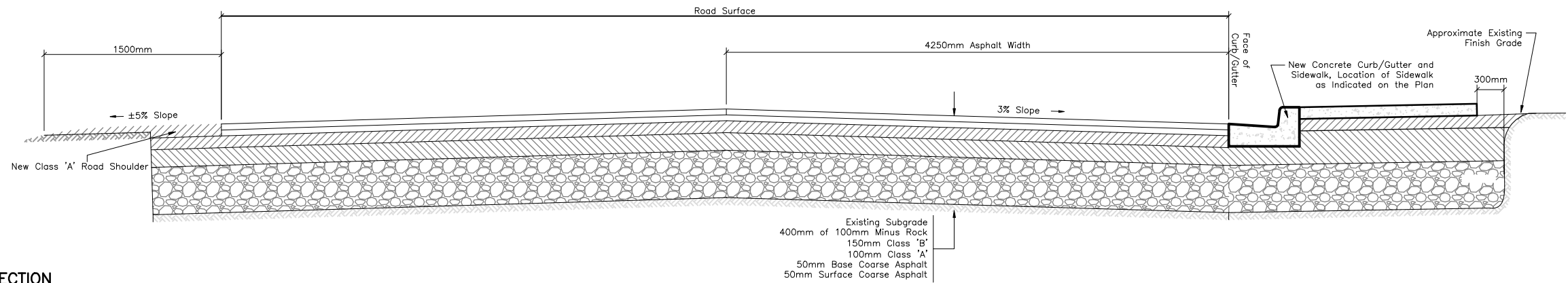
TYPICAL ROAD SECTION STA. 0+068.50 TO STA. 0+113.00
