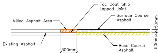
SHI LAP JOINT - NEW ASPHALT TO EXISTING ASPHALT
